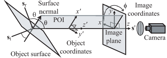
Fig. 2 Reflected and transmitted light observed by the camera.
