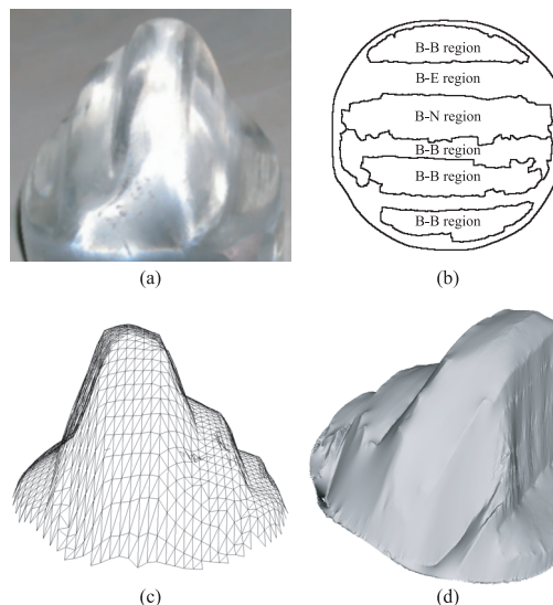
Fig. 20 Measurement result of transparent mountain-shaped object: (a) Real image, (b) region segmentation result, and (c) and (d) rendered image.
