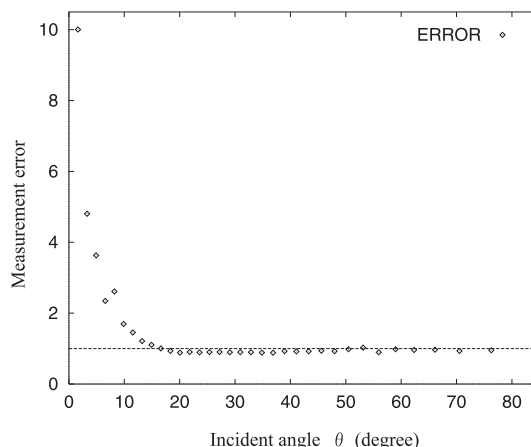
Fig. 15 Error characteristics of the spherical object.
