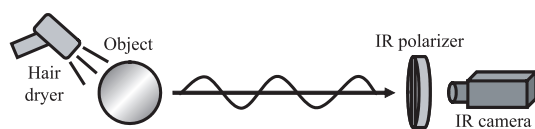
Fig. 13 Experimental setup for infrared light.
