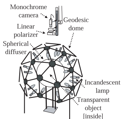
Fig. 12 Experimental setup for visible light.
