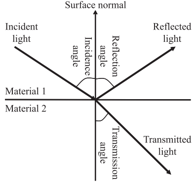
Fig. 1 Reflection, refraction, and transmission.
